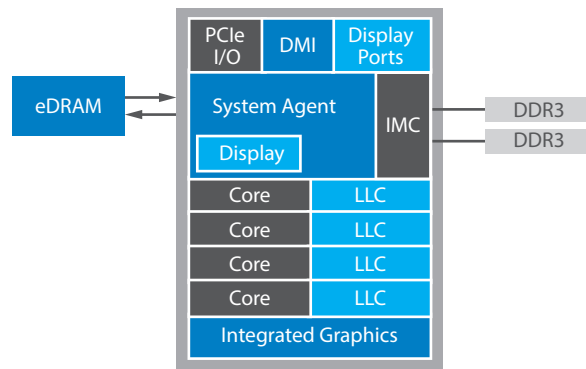
Figure 3. Intel® processor and processor graphics elements.
