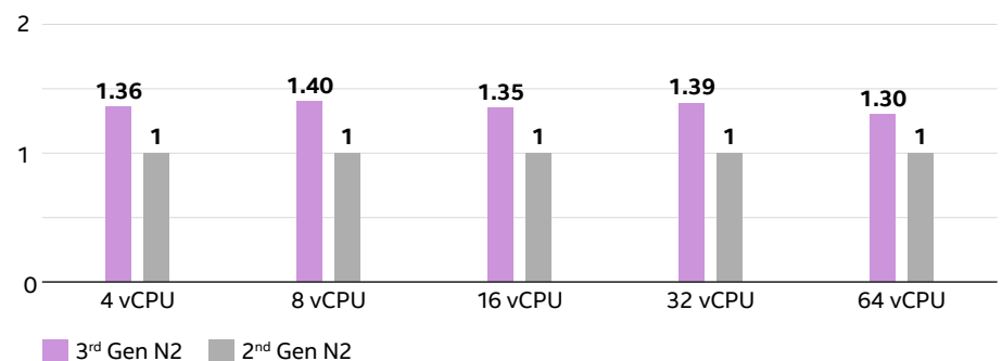
Figure 1. Relative SPECjbb 2015 Max-jOPS results for five sizes of newer Google Cloud N2 VMs and older N2 VMs.
