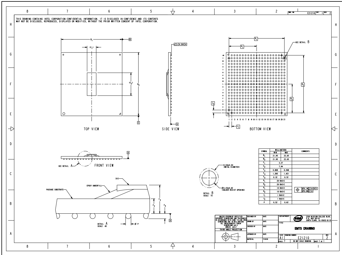
Figure 5. Package Mechanical Drawing
