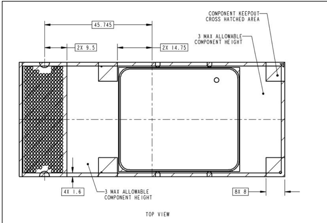
Figure 4-4. Processor Package Top-Side Components Height Dimensions
