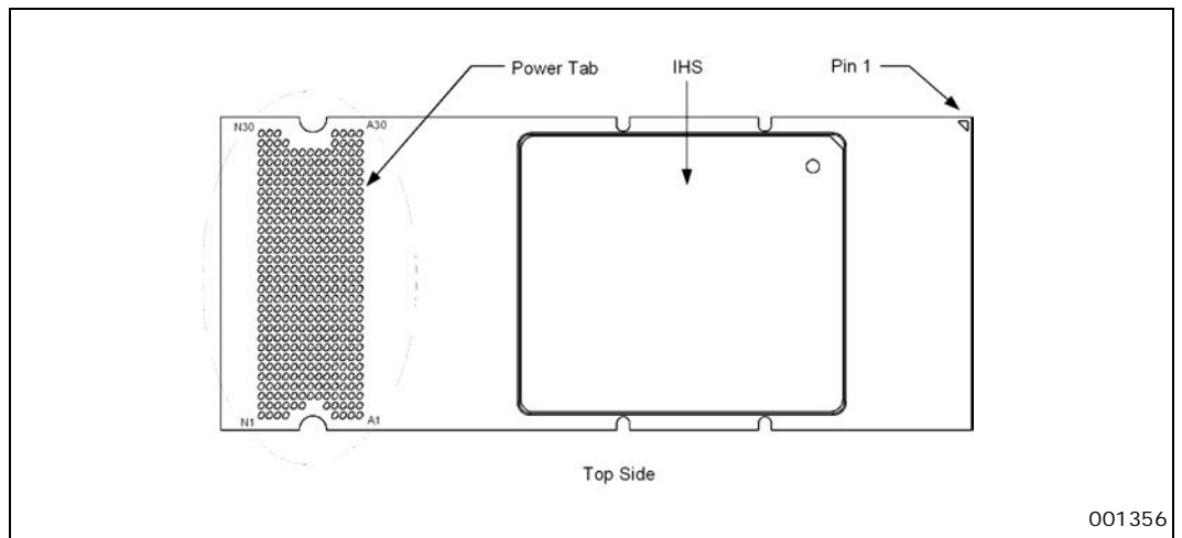
Figure 2-4. Processors Power Tab Physical Layout
