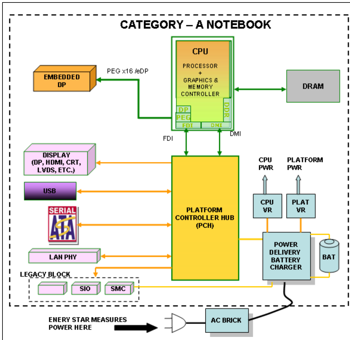
Figure 3. Typical CAT A Notebook System (Integrated graphics, UMA Memory)
