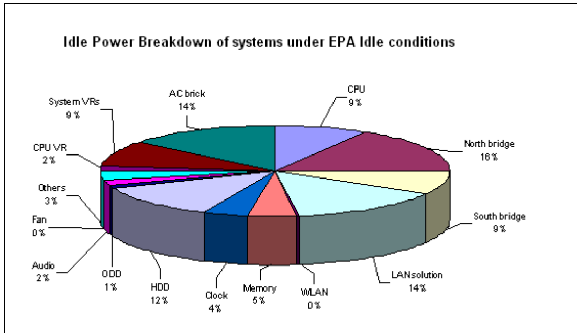
Figure 7. Typical Notebook Idle Power Breakdown
