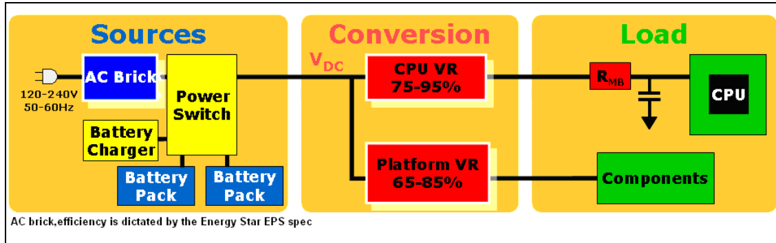
Figure 5. Notebook Power Delivery System
