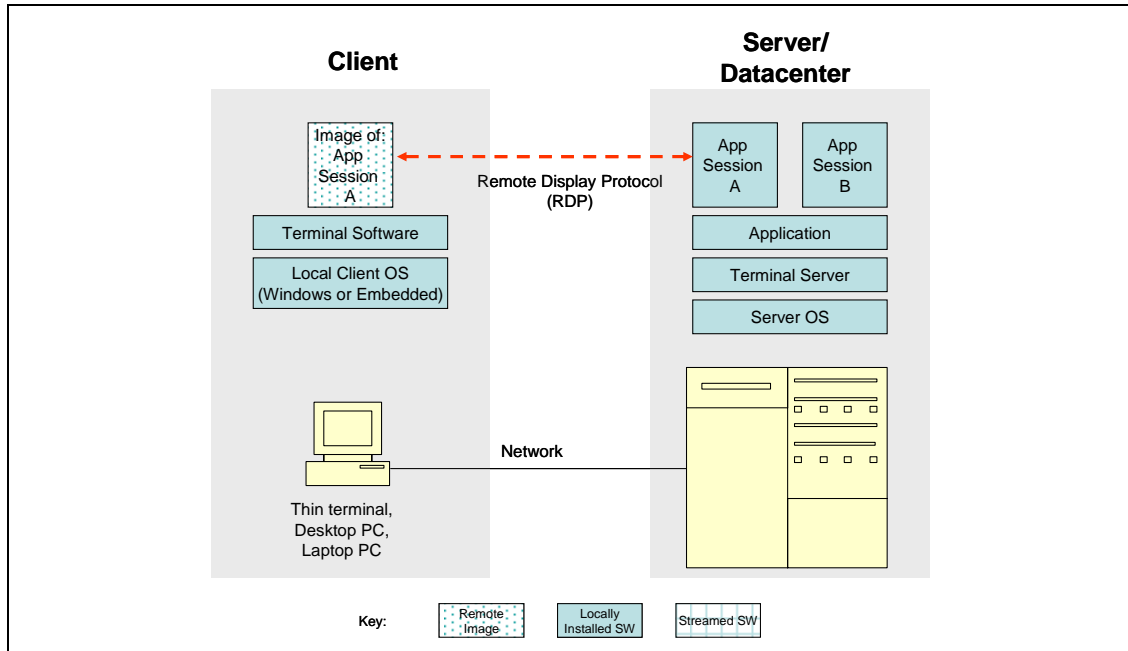
Figure 21. Architecture - Terminal Services
