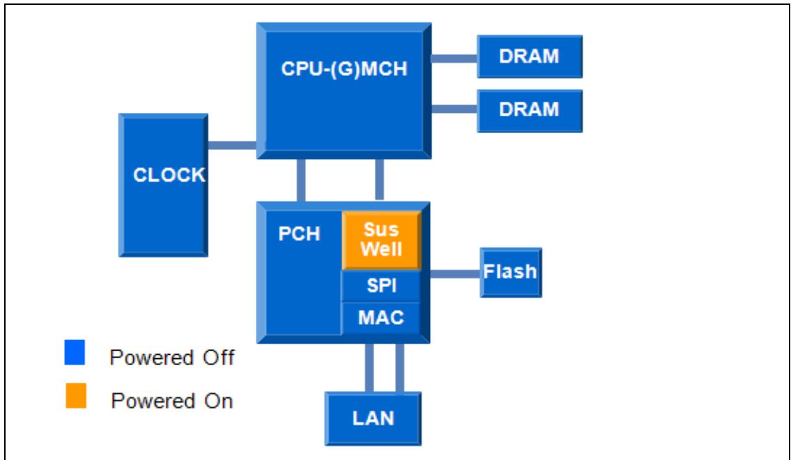
Figure 18. Off (S5) Mode System Power State Example
