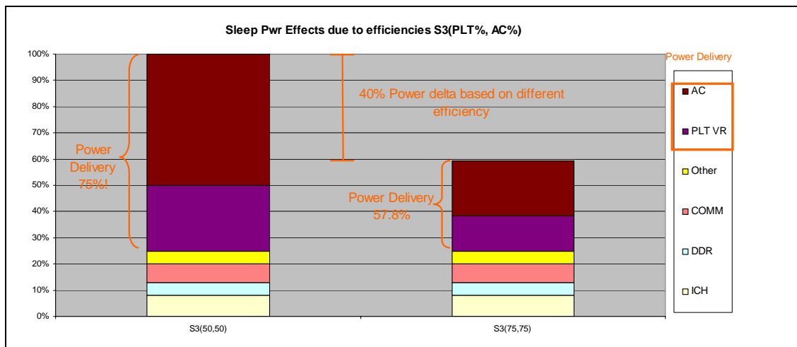
Figure 10. Sleep Power distribution across efficiencies
