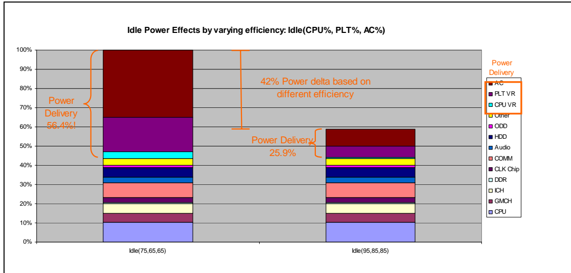
Figure 9. Idle Power distribution across efficiencies
