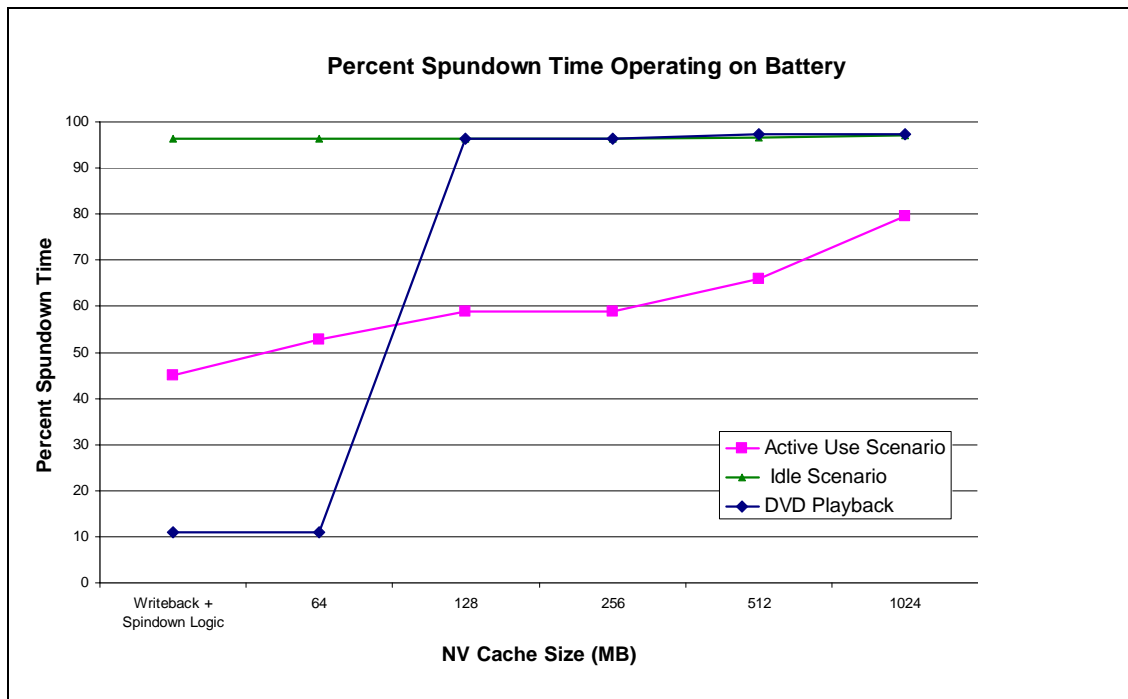
Figure 12. Percent Spundown Time Operating on Battery
