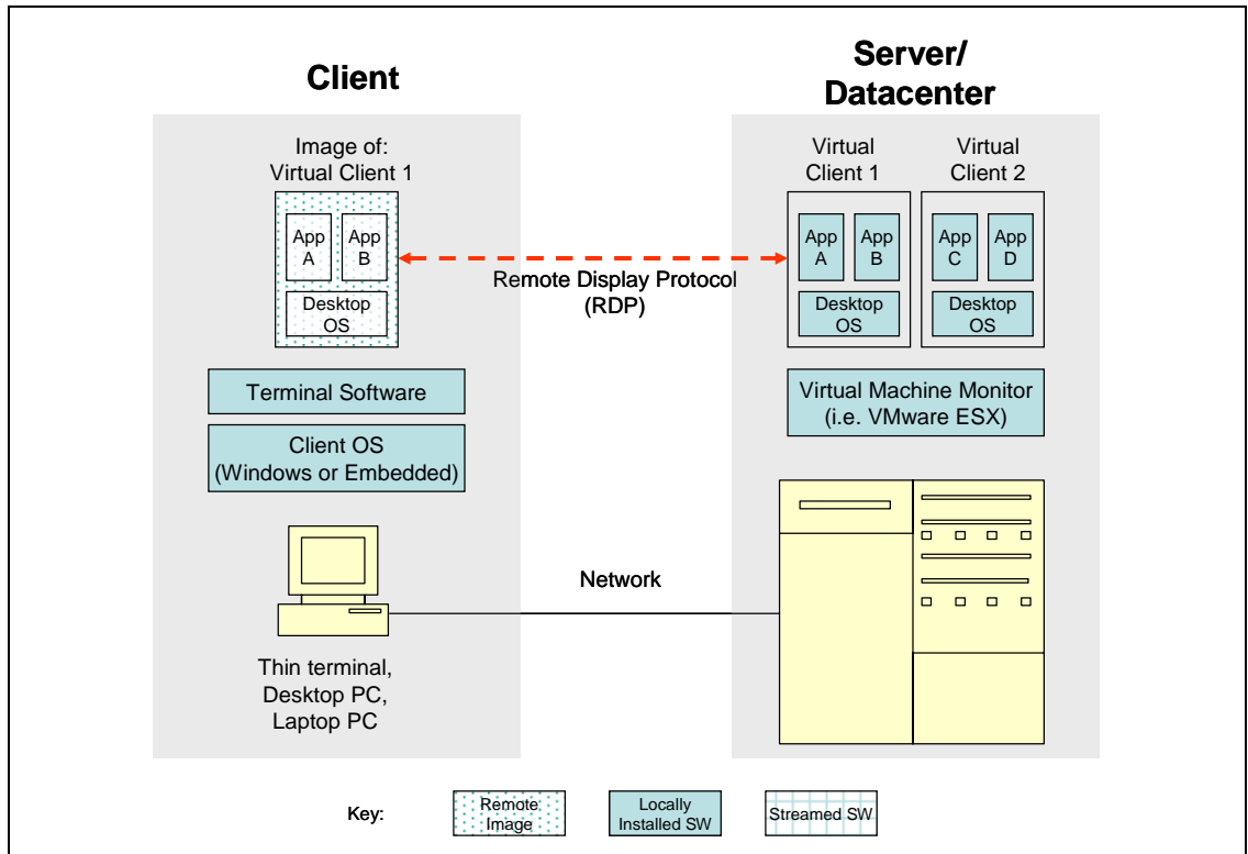
Figure 22. Architecture – Virtual Hosted Desktop
