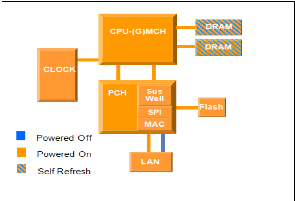
Figure 16. Idle State System Power State Example
