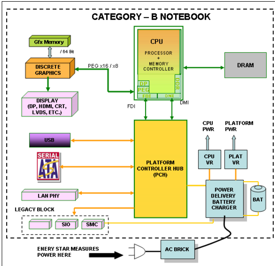
Figure 4. Typical CAT B Notebook (discrete graphics)
