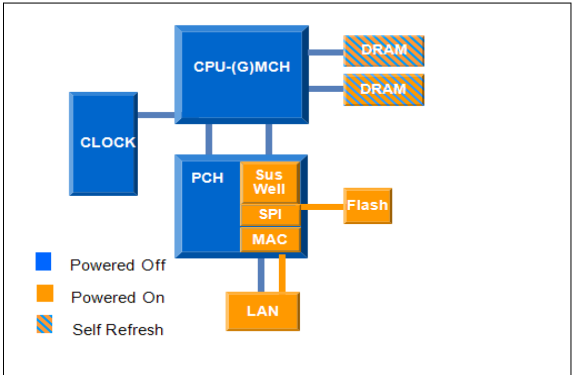
Figure 17. Sleep (S3) Mode System Power State Example
