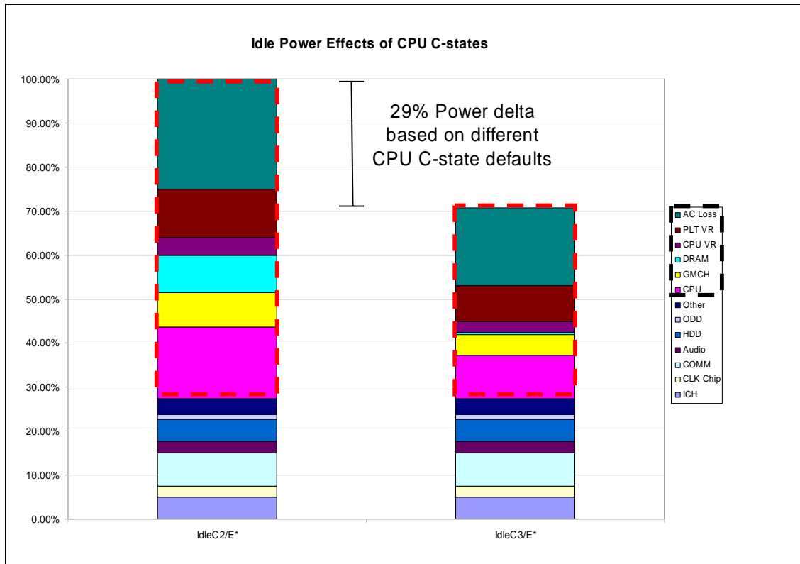
Figure 11. Idle Effects of Low Power States
