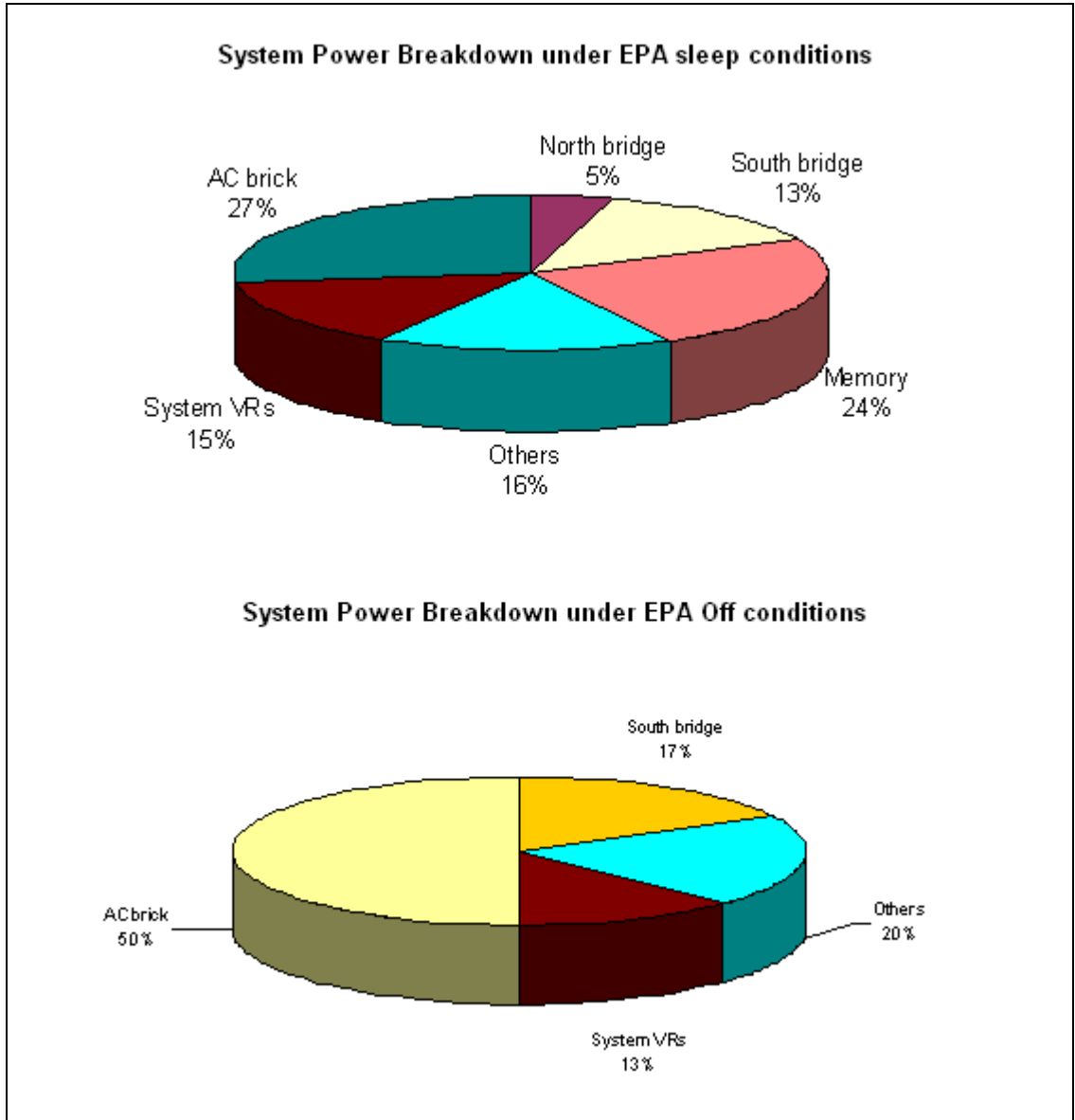
Figure 8. Typical Notebook Sleep and Off Power Breakdown
