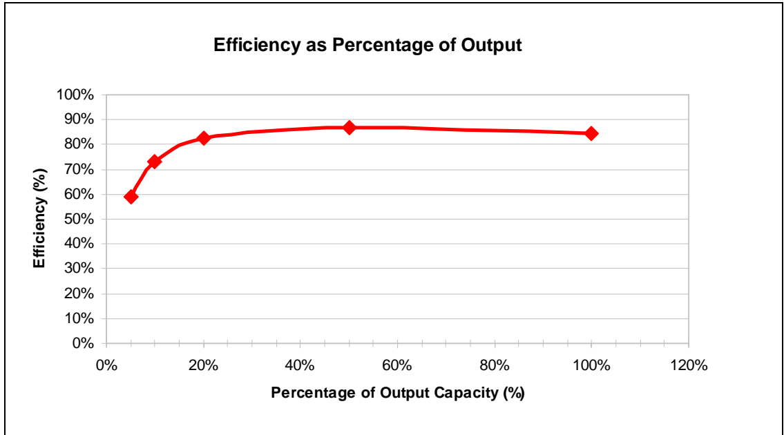
Figure 13. PSU Efficiency as Percentage of Output
