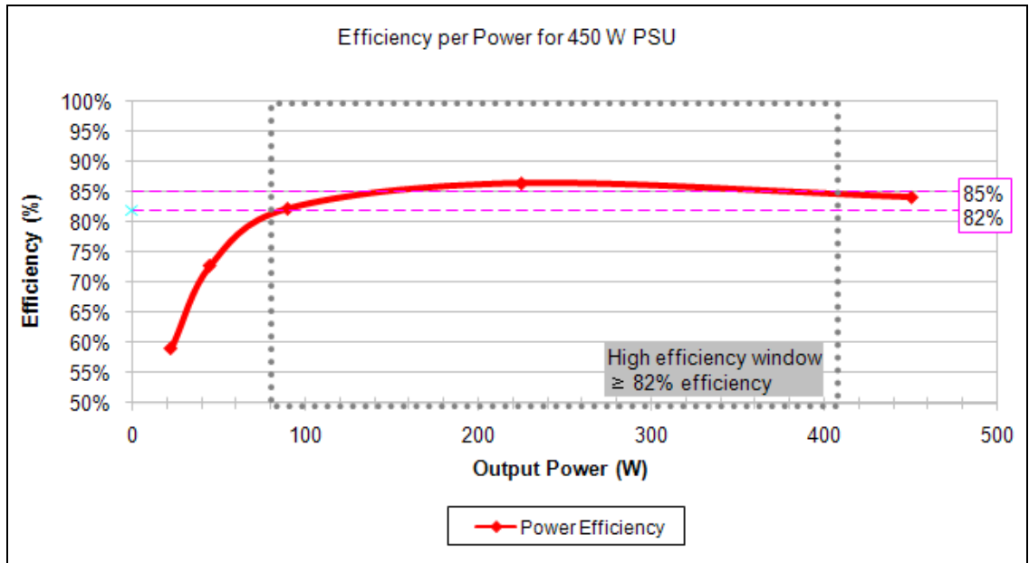
Figure 14. PSU Efficiency per Power for 450 W PSU
