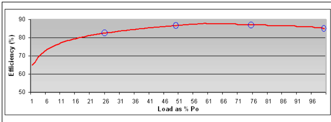
Figure 6. Example AC Brick Efficiency over Different Loads
